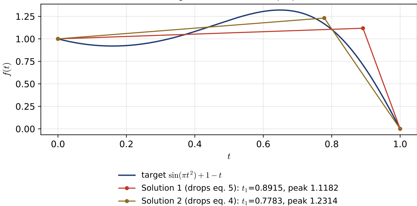
(c) two-segment inversion of \sin(\pi t^2) + 1 - t
