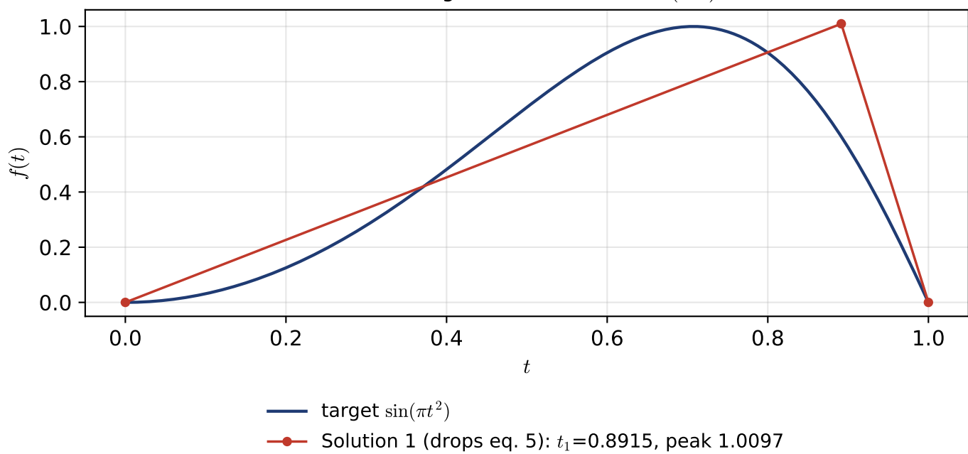
(b) two-segment inversion of \sin(\pi t^2)
